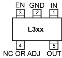
MIC5233 5-Pin SOT23 (Top View)
