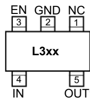
MIC5233 5A-Pin SOT23 (Automotive Specific) (Top View)
