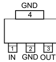
MIC5233 3-Pin SOT223 (Top View)
