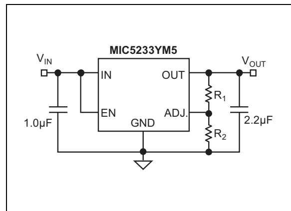
FIGURE 4-1: Adjustable Voltage Application.
